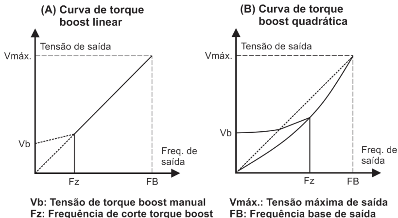
Fig.6-3 Torque boost
