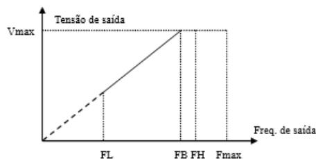
Fig.6-2 Fmax/FB/Vmax0V
