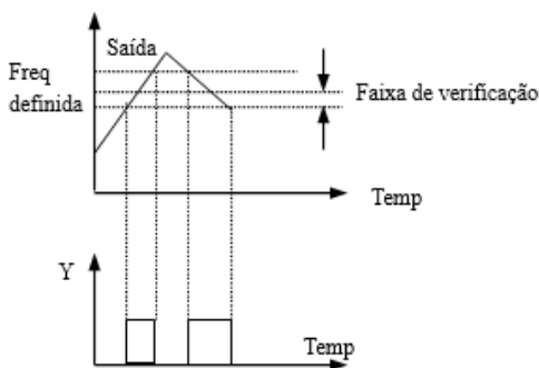
Fig.6-26 Sinal de freq. atingida
